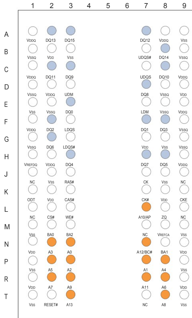
Figure 1: 96-Ball FBGA Ball Assignments (Top View), JT
